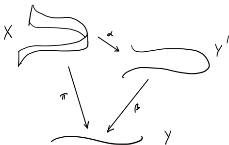
FIGURE 30.4. Stein Factorization
